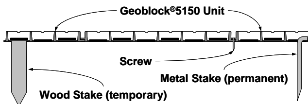
Figure 6 Anchoring Possibilities
